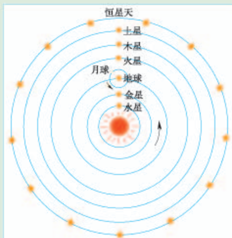
图1.15 “日心说”示意
